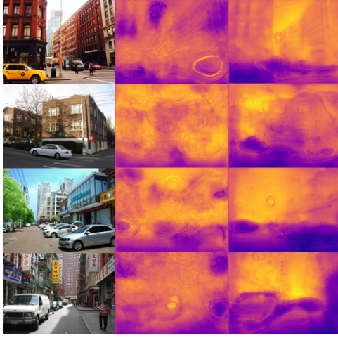
Figure 11: Left to Right: RGB Input Images (Newly Seen, City), U-Net Depth Predictions (20 Epochs), W-Net Connected Depth Predictions (20 Epochs).
